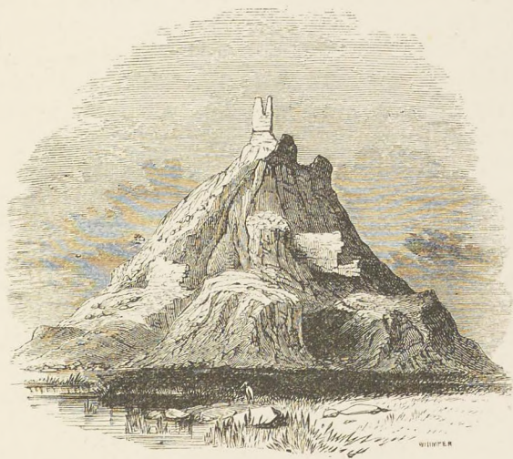
BIRS NIMROUD.
